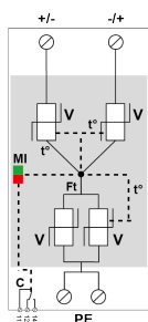
V: High-energy varistor Ft: Thermal fuse C: Remote signal contact t*: Thermal disconnection system MI: Mechanical disconnection indicator
